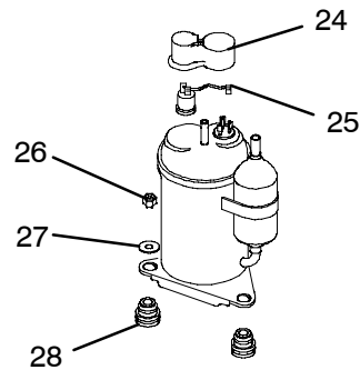
ITEM 23 - COMPRESSOR ASSEMBLY
